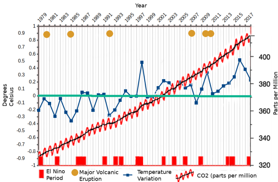
UAH satellite-based Lower Tropospheric (LT) temperature dataset and atmospheric concentration of Carbon Dioxide; 1979 to present
